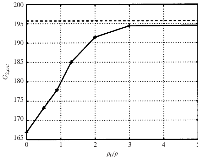
FIGURE 12. Critical values of Galileo number at the onset of the Hopf secondary bifurcation vs. the sphere density.
